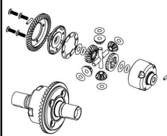
HI903-104 Diff. unit
