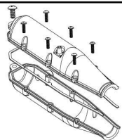
HI903-041 Exhaust pipe set
