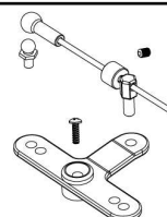
HI903-045 Throttle servo horn and linkage set
