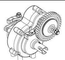
HI904-011 Gearbox unit
