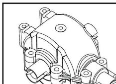
HI903-020 Diff. gearbox unit
