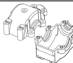
HI903-098 Diff. gearbox bulkhead-upper/lower
