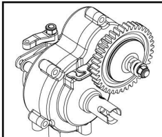
HI903-047 Centre gearbox unit
