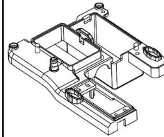
HI903-039 Upper deck -centre
