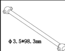
HI904-009 Dogbone-Fr
