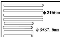
HI903-024 Front suspension arm pin-short 4pcs HI903-025 Suspension arm pin-long 4pcs
