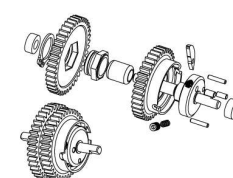
HI903-103 Gear-40T/37T
