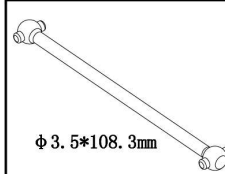
HI904-010 Dogbone-Rr
